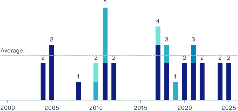
Number of Events above $10B
