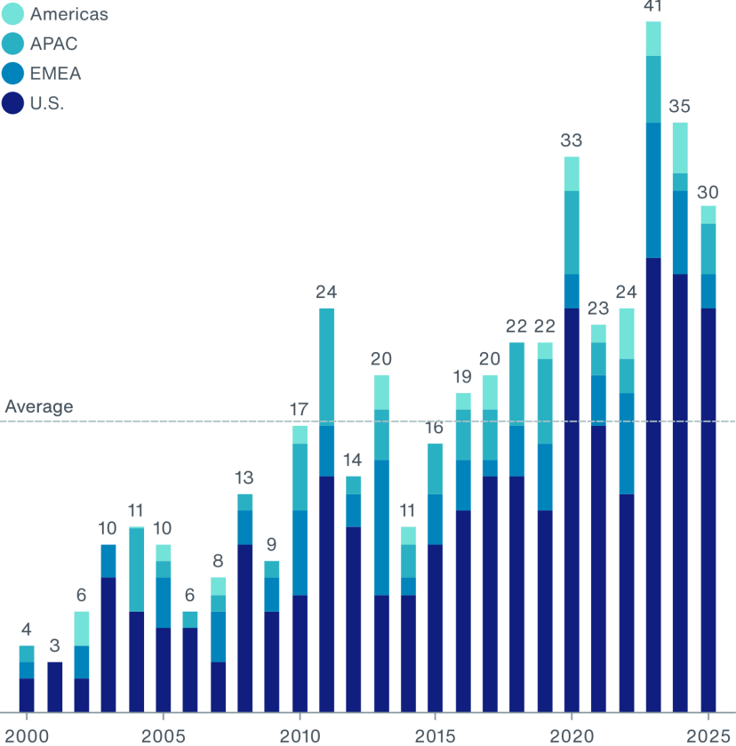
Number of Events above $1B
