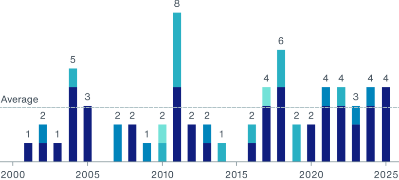
Number of Events above $5B
